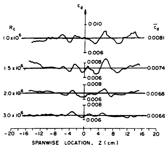
Fig. 2 Spanwise variation in profile drag coefficient at Reynolds numbers ranging from 1-3 \times 10^6 (Mueller, 17 adapted from Althaus 9 ).
