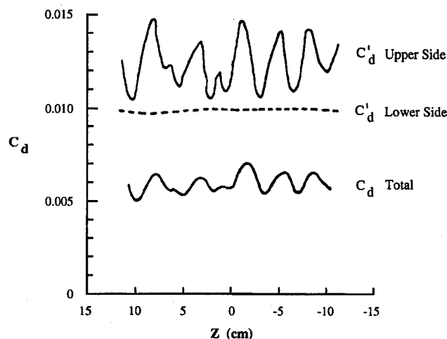
Fig. 3 Spanwise variation in profile drag for the FX 78-K-140 airfoil at Re = 2.5 \times 10^6 and \alpha = 3 deg. Wake traverses performed at trailing edge of model (adapted from Althaus 9 ).
