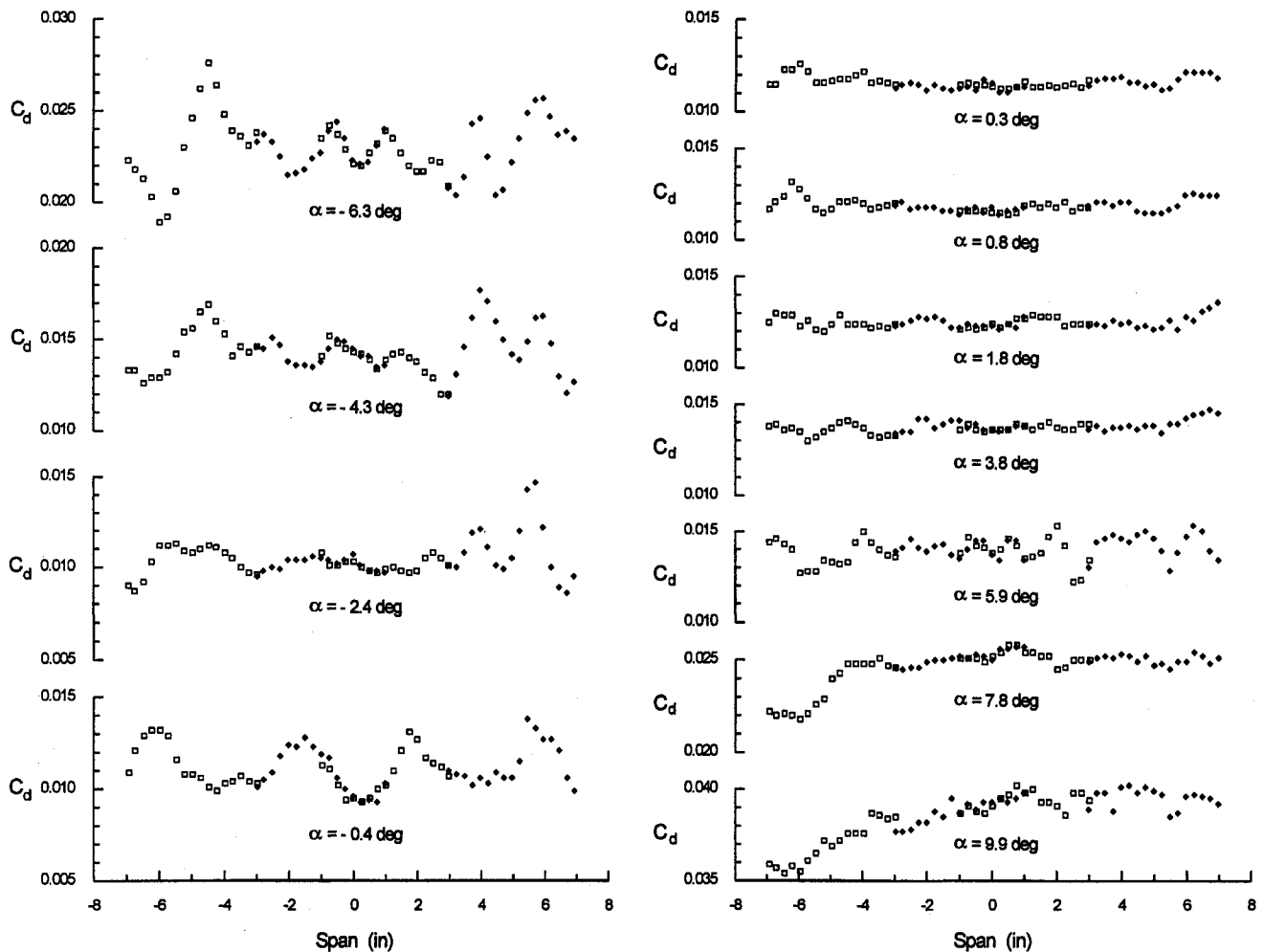
Fig. 9 Spanwise drag results for the E374 airfoil at Re = 2 \times 10^4 .
